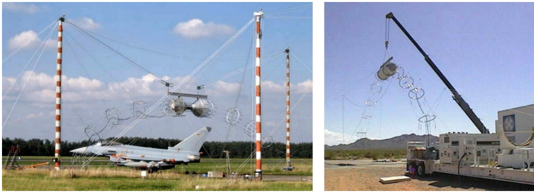
Fig. 4.11. Hybrid-type simulators: stationary (left), mobile (right).
