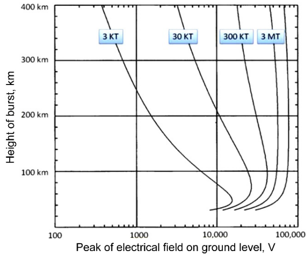
Fig. 3.11. Variations in the intensity of HEMP exposure.
