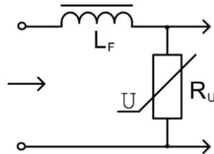
Fig. 4.15. Equivalent circuit for ferrite filter ( L_F ) and varistor ( R_U ) connection.
